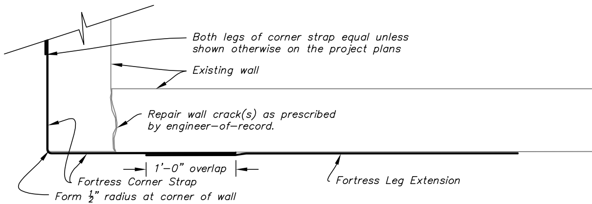
1 PLAN VIEW SCALE: 1"=1'
