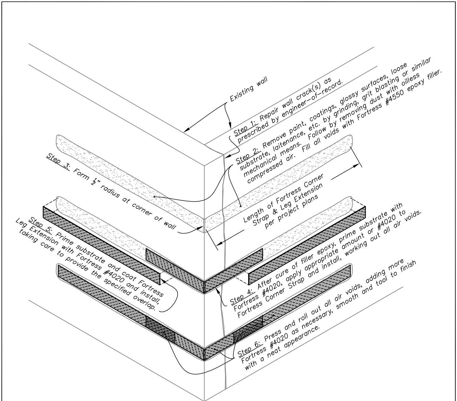
3 ORTHOGRAPHIC VIEW SCALE: None
